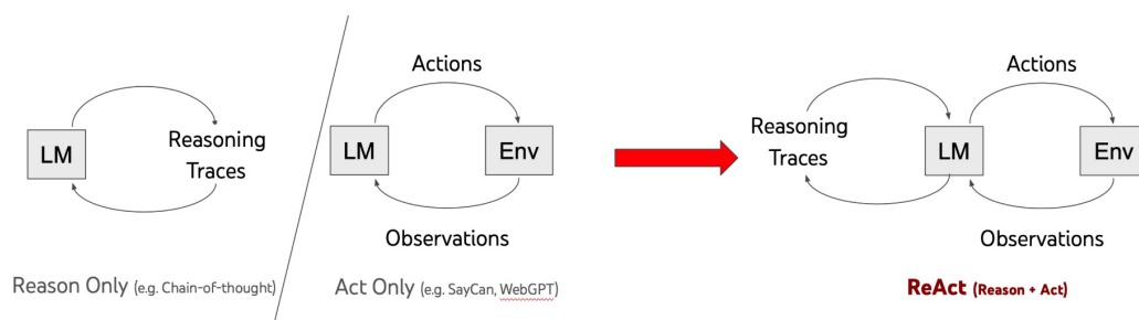
ReAct-LLM
