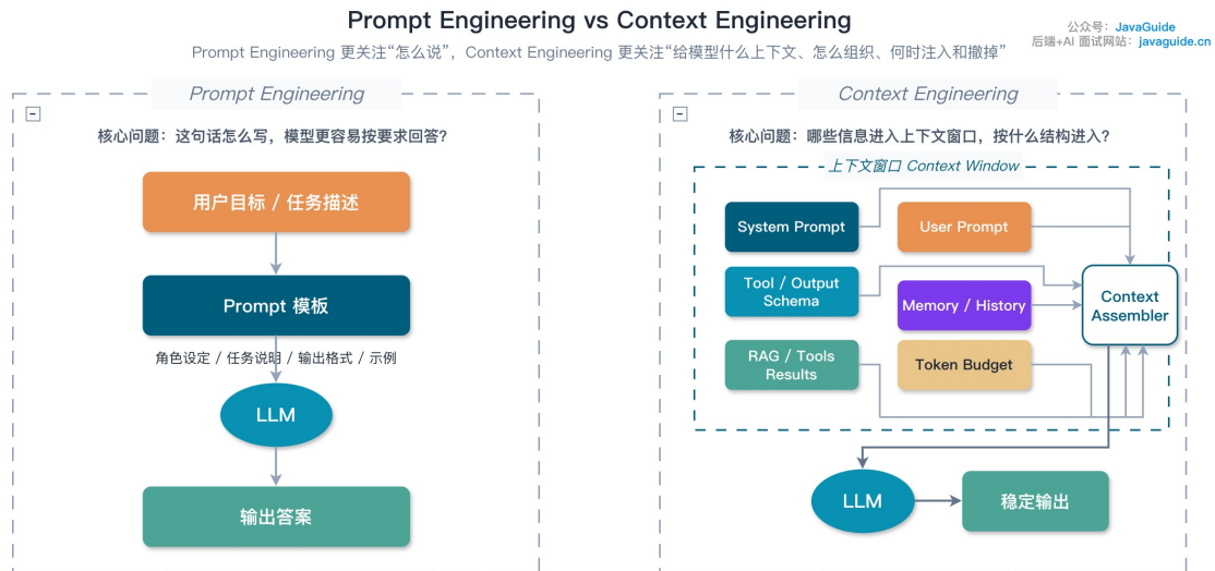
Context Engineering 和 Prompt Engineering 差别
